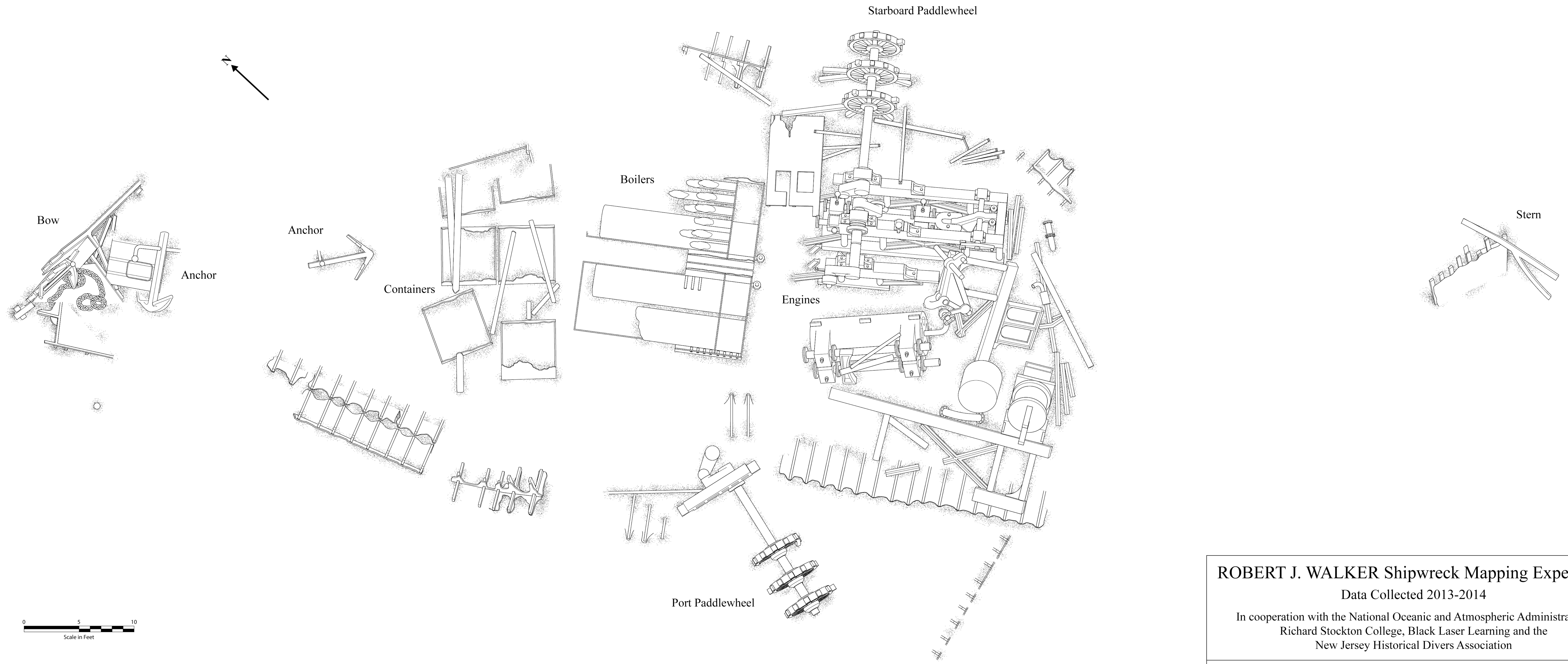
ROBERT J. WALKER Wrecksite - Plan View
